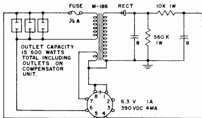
POWER SUPPLY MODEL D-8
