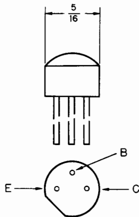
⑧ TO-105
