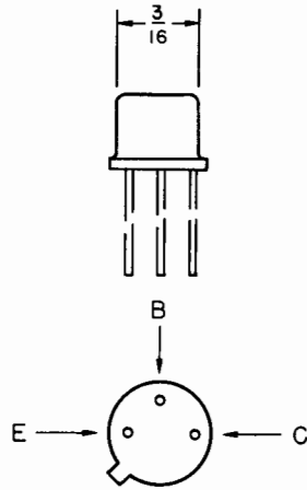
② TO-18
