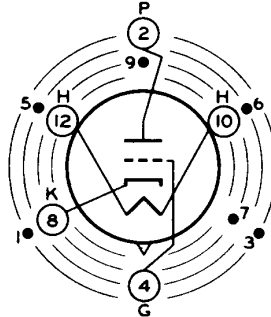
INDEX=LARGE LUG ●=SHORT PIN; IC-DO NOT USE
